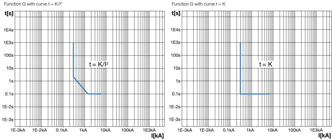
Figure 9: Trip curves of function G
